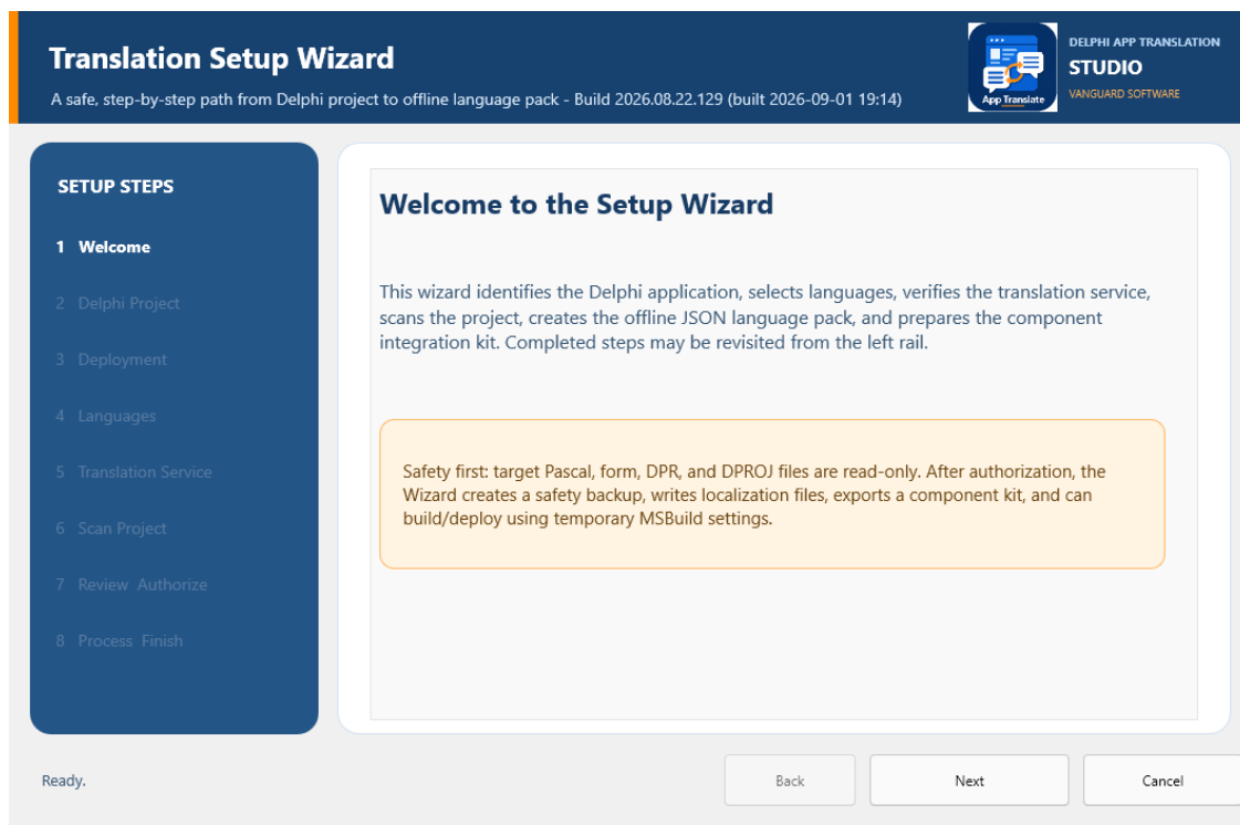
Figure 10-1. Welcome page.
